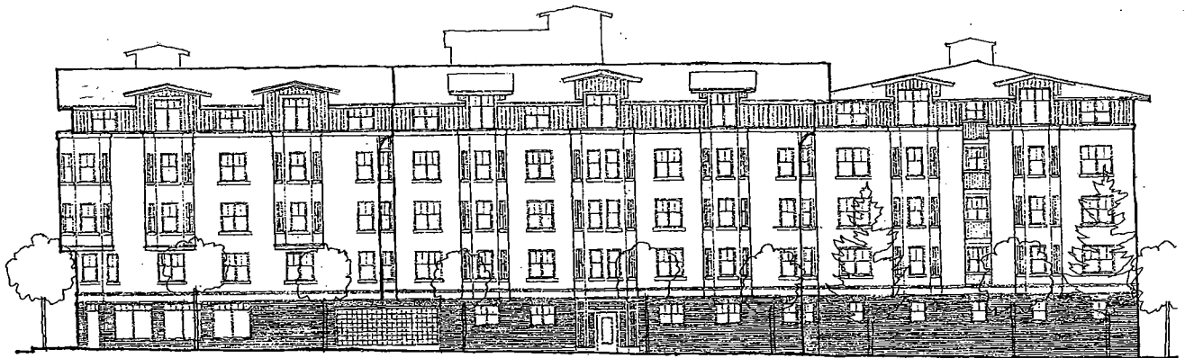
2 NORTH ELEVATION (BUILDING ON BERKELEY WAY)
